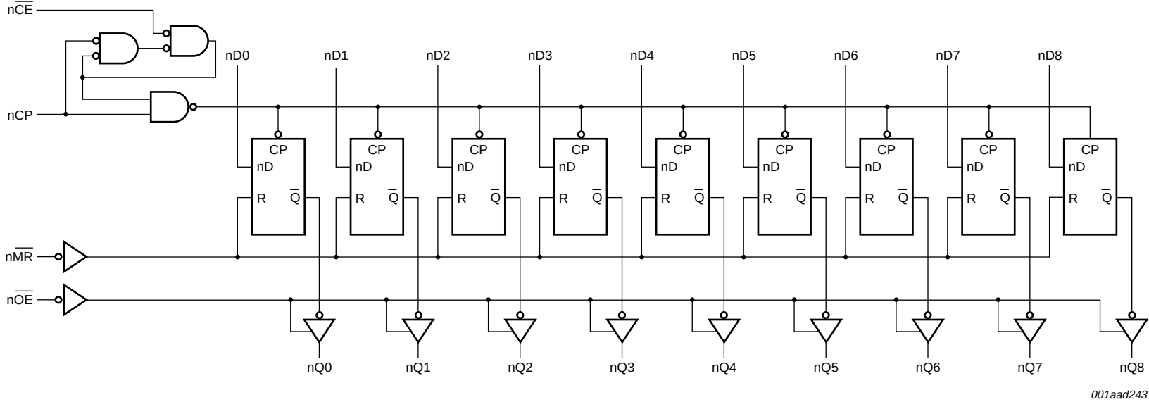
Fig 4. Logic diagram
